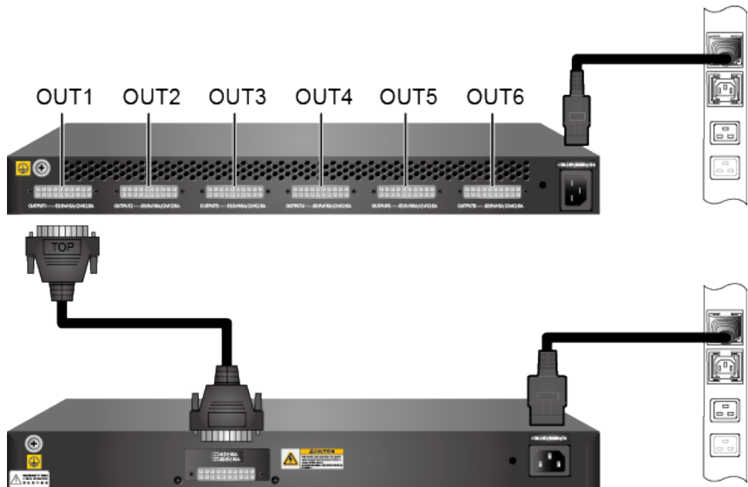
Figure 3-2 Connecting an RPS1800 to an S5720S-S
