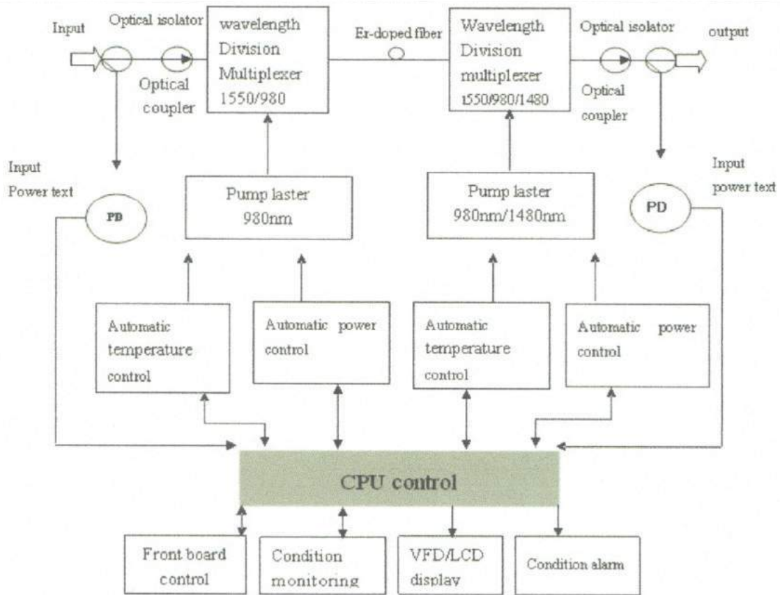
Diagram of erbium-doped fiber amplifier
