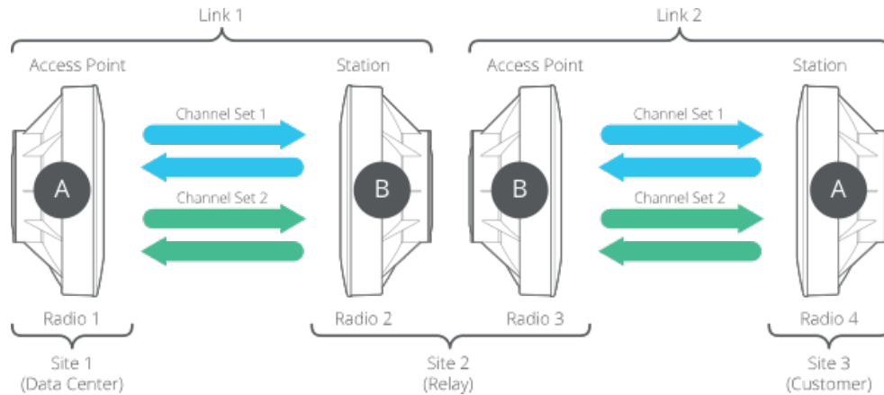
Figure 5 – Example PTP Link (Multi-hop)
