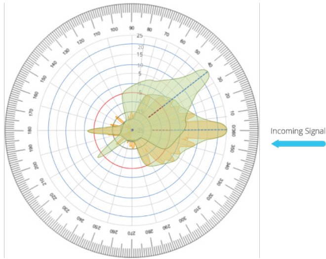
Figure 13 – Two Overlapping B5 Antenna Patterns
