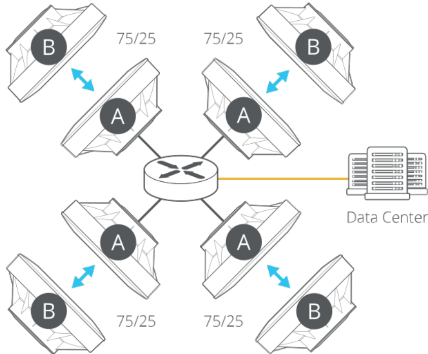
Figure 11 – Star Network with 75/25 Traffic Split
