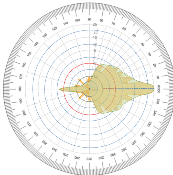
Figure 12 – B5 Antenna Pattern on 360° Compass
