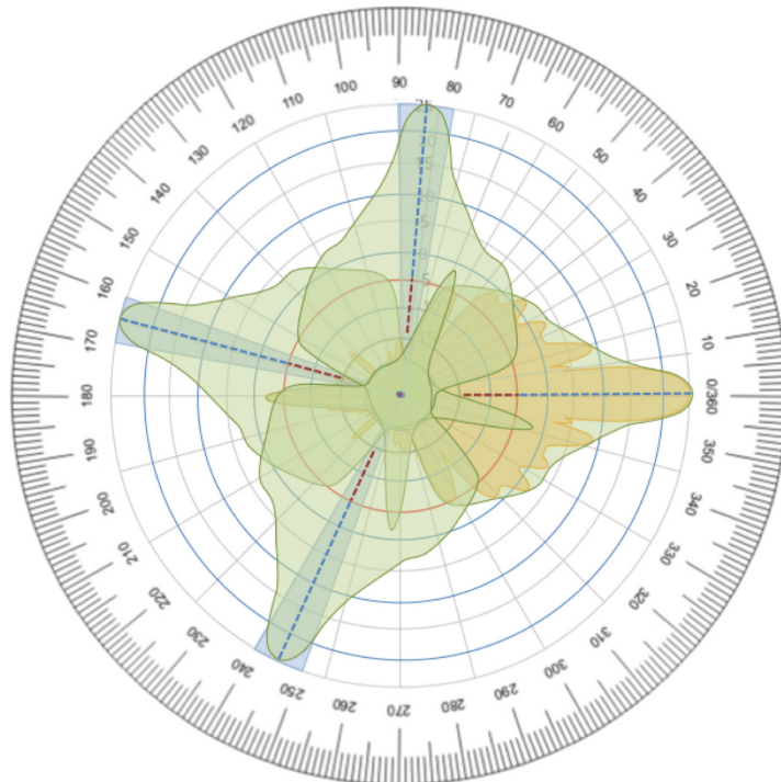
Figure 16 – Four Non-Overlapping B5 Antenna Patterns
