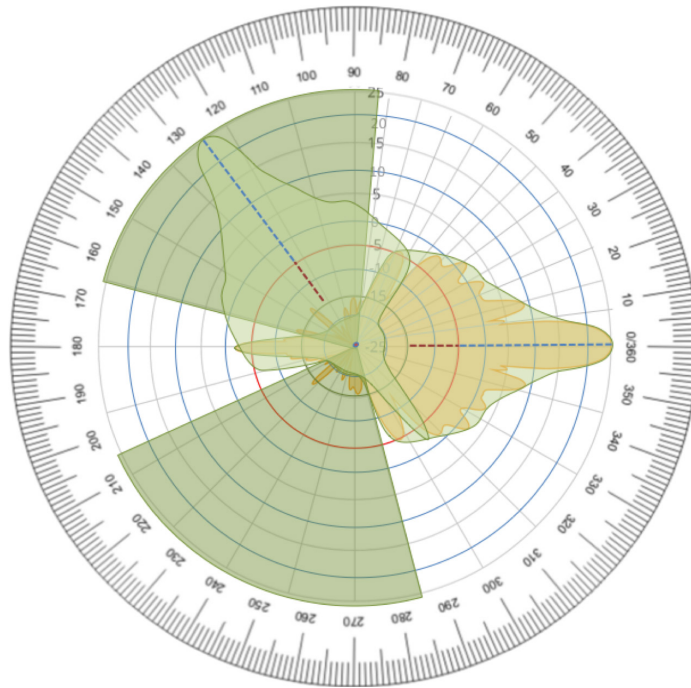
Figure 14 – Two Non-Overlapping B5 Antenna Patterns
