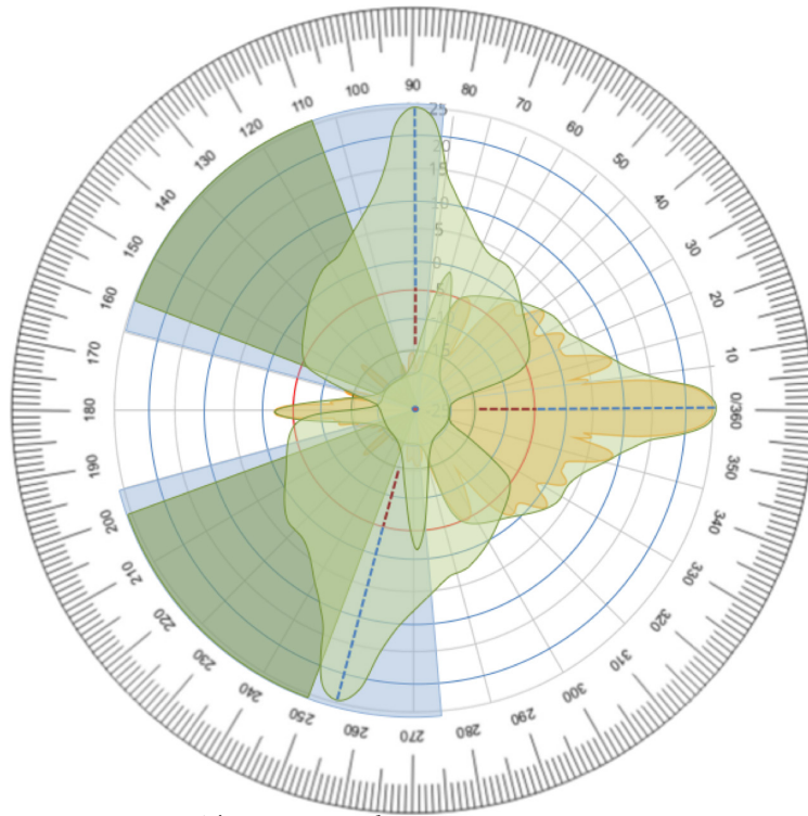
Figure 15 – Three Non-Overlapping B5 Antenna Patterns
