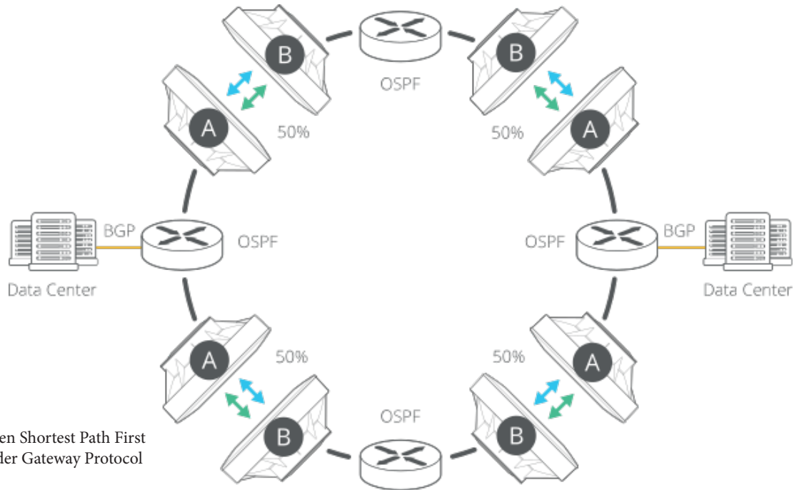
Figure 8 - Ring Topology (50/50 Traffic Split)
